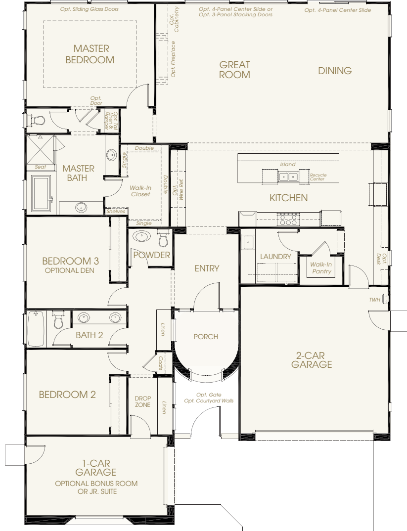
OPTION: Bonus Room in lieu of 3-Car Garage (Adds 226 Sq. Ft.)
